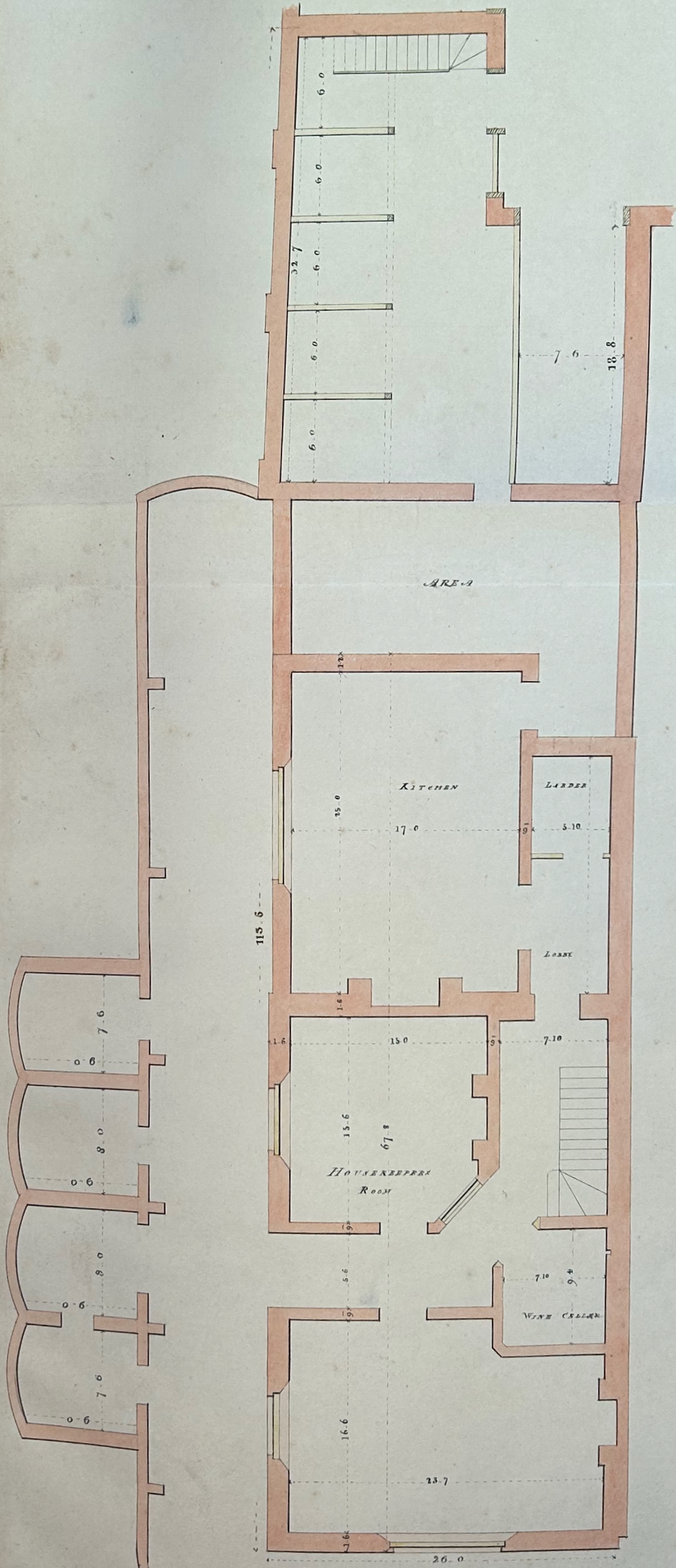
BASEMENT PLAN CORNER HOUSE SOUTH SIDE EATON PLACE
